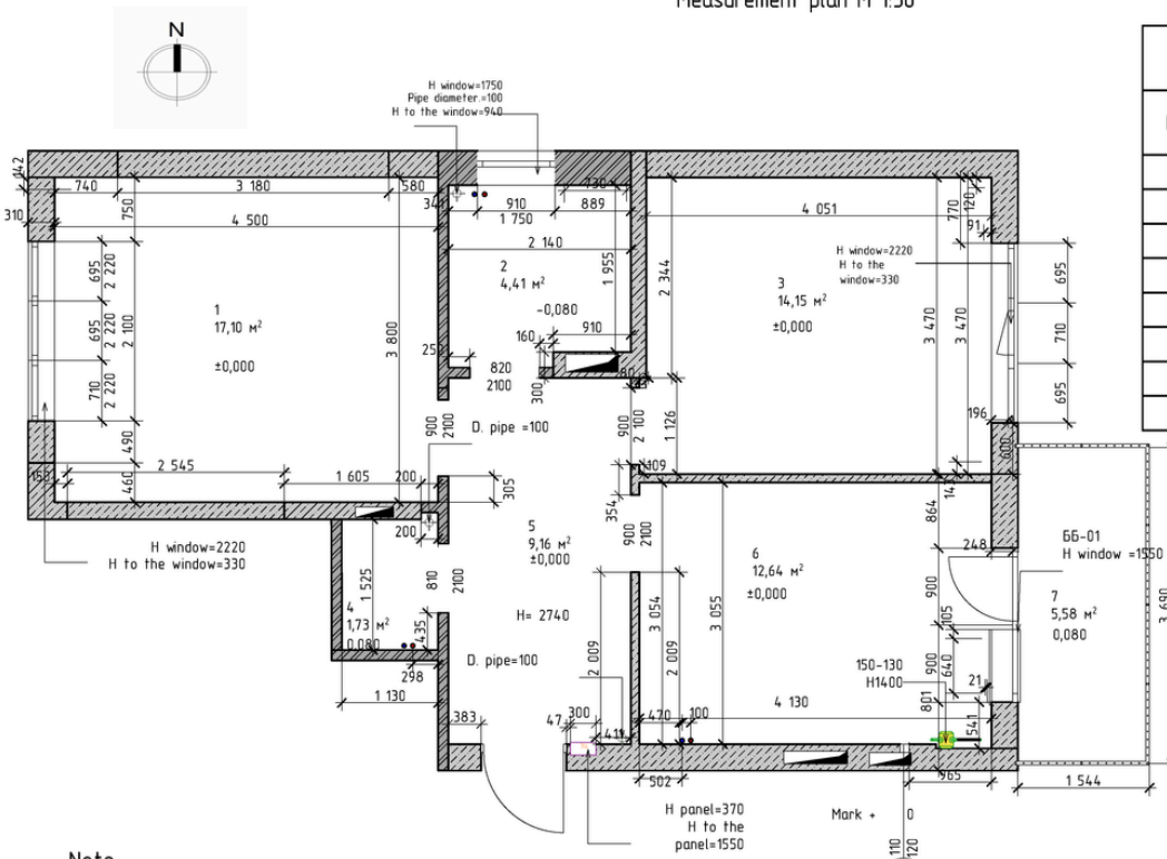
Measurement plan M 1:50
